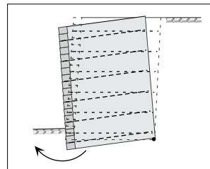
Figure 4:15 Reinforced Wall Bearing Failure
