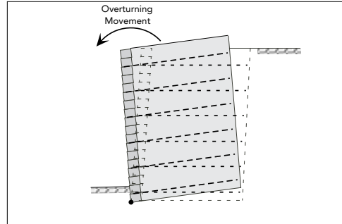
Figure 4:13 Reinforced Wall Overturning
