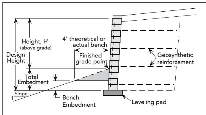
Figure 4:2 Sloping Toe
