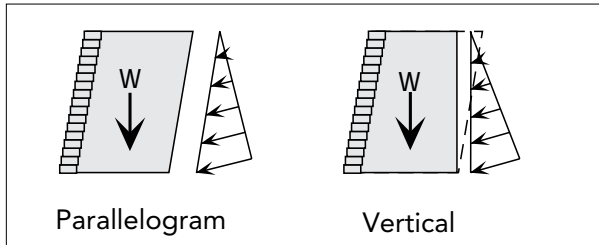
Figure 4:8 Design Options
