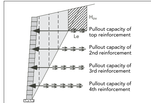
Figure 4:19 Pullout Diagram
