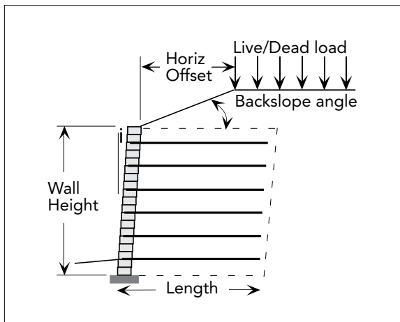
Figure 4:1 Design Section
